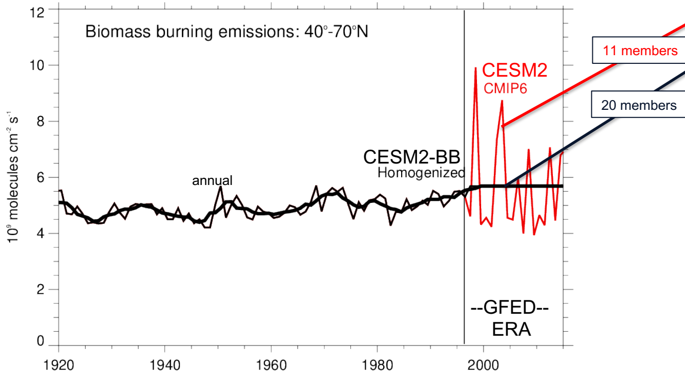
Above: CMIP6 prescribed biomass burning (BB) emissions – a large increase in variability for GFED.
