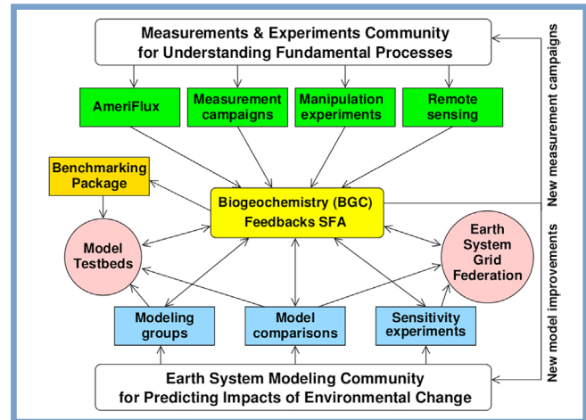
Figure 1: The Biogeochemistry (BGC) Feedbacks Scientific Focus Area (SFA) brings together the modeling and the measurements communities to systematically assess model fidelity using best available observations through an open source benchmarking package.
