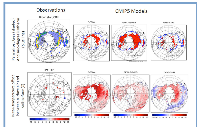
Figure 2: CMIP5 models exhibit a large inter-model spread in permafrost properties, including permafrost area and mean temperature across the atmosphere–soil interface. However, none of these individual variations was strongly related to modeled permafrost susceptibility to warming. Figure adapted from Koven et al. (2013).
